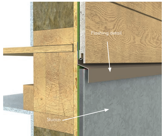
Fig.33 - Horizontal joint over stucco
