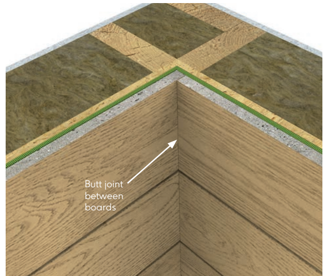
Fig. 12 - Internal corner butt joint
