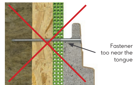
Fig.18 - Fastener depth and position
