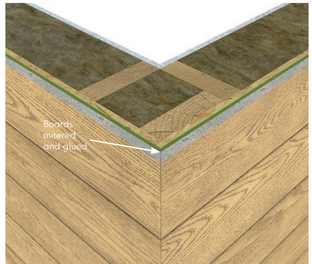
Fig. 13 - External corner miter joint
