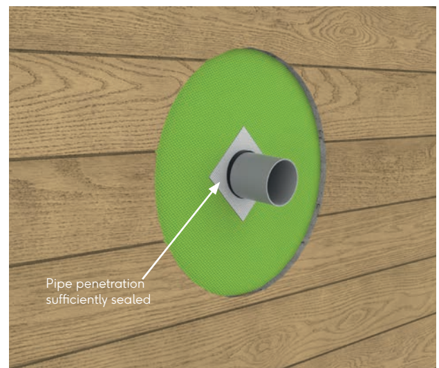
Fig.30 - Wall penetration
