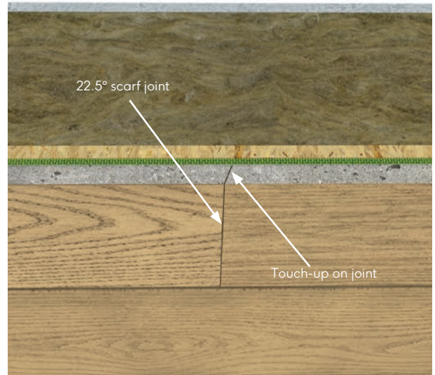
Fig.21 - Board joint
