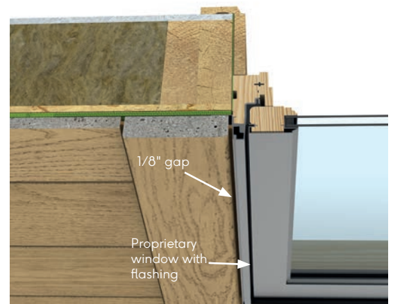
Fig.26 - Window jamb with Enhanced Grain
