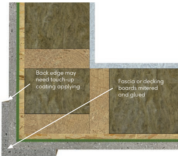
Fig. 14 - Mitered corner top view
