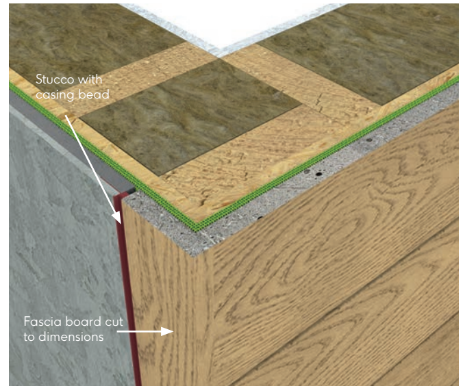
Fig.32 - Corner detail to stucco
