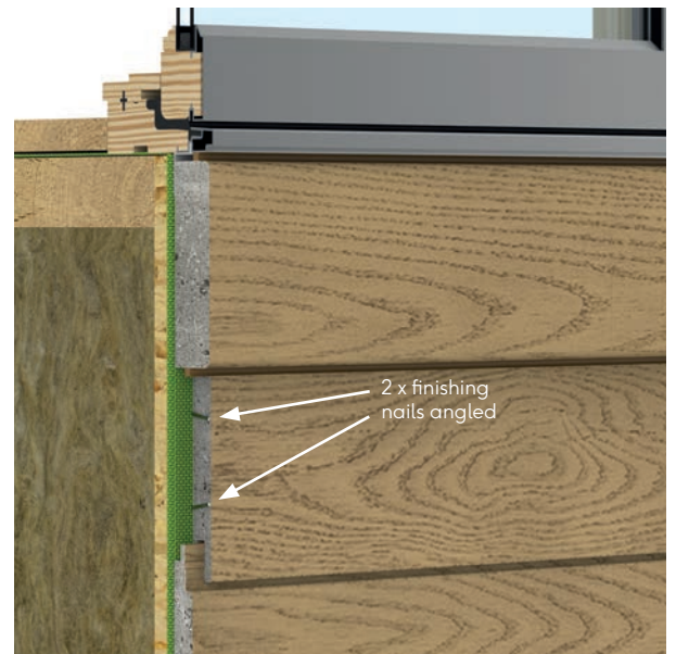
Fig.20 - Typical finishing nail detail - Window sill
