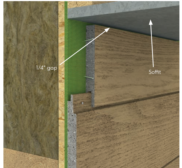
Fig. 19 - Wall head
